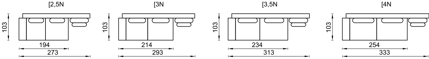
CORNER ELEMENT ELEMENT DE COIN
